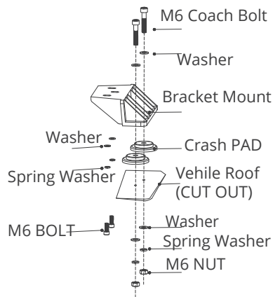
PLASTIC BRACKET MOUNTING (OPTIONAL ACCESSORY) KIINNITYSJALAT / PLASTFÄSTE / PLASTBRACKETT
