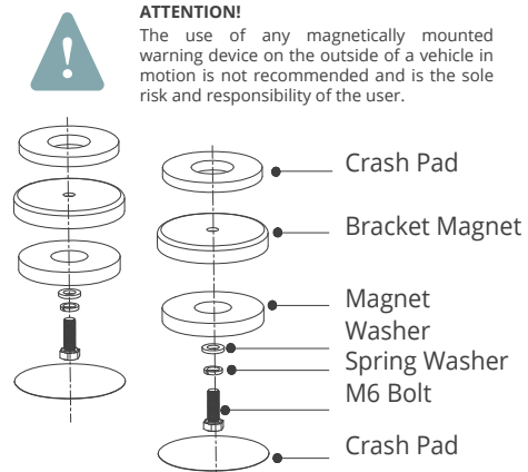
TEMPORARY MAGNETIC MOUNTING (OPTIONAL ACCESSORY) MAGNEETTIKIINNITYS / MAGNETISK MONTERING
